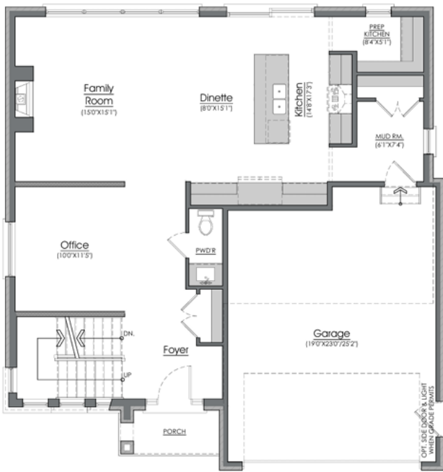
MAIN FLOOR PLAN 1074 SQ. FT. (TOTAL 2324 SQ.FT.)
