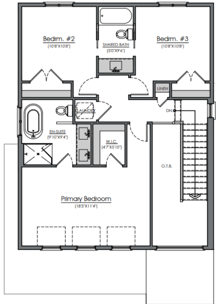
UPPER FLOOR PLAN 990 SQ. FT. inc. 138 SQ.FT. OPEN SPACE
